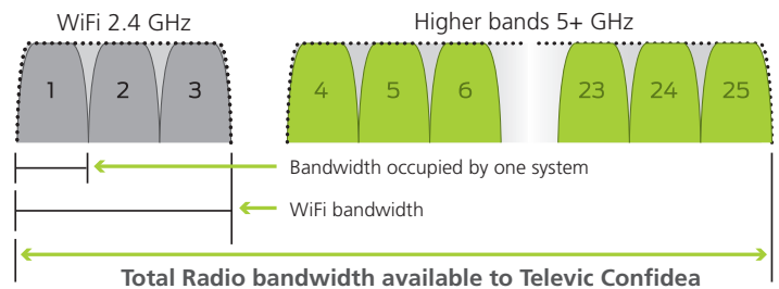
Televic Confidea "Quad-band" system
